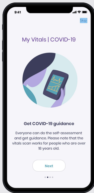
GUIDANCE OVERVIEW
